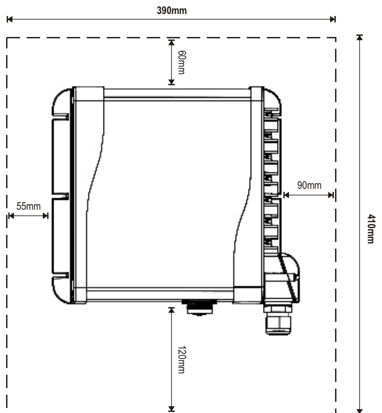
Diagram 2 - Front View
